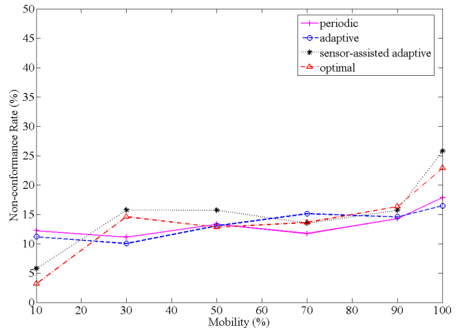
Figure 7. Non-conformance rate v.s. different mobility levels given an application-specified error tolerance of 7 meters.
