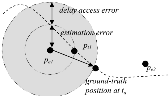
Figure 1. Sampling error sources
