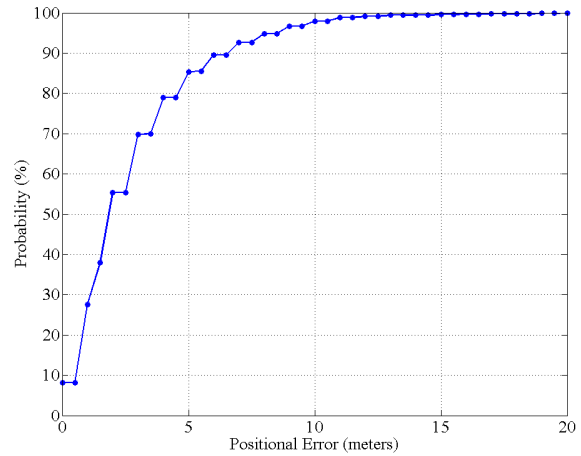
Figure 3. Position error cumulative probability distribution
