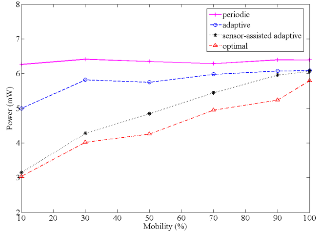
Figure 6. Power consumption given different mobility levels under an application-specified error tolerance of 7 meters
