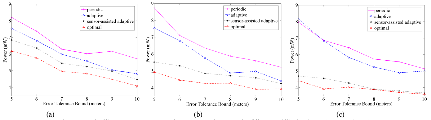
Figure 8. Tradeoff between power consumption and error tolerance under different mobility levels (70%, 50%, and 30%).
