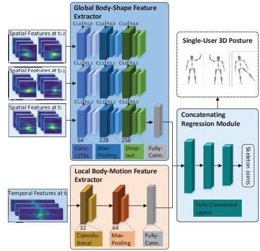
Figure 7: Neural network structure of m 3 Track.
