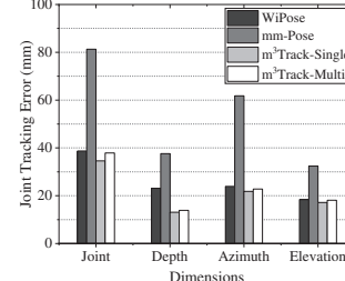
Figure 18: Joint tracking errors for m^3Track , WiPose , and mm-Pose .
