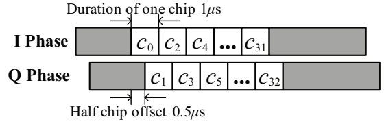
Figure 5: O-QPSK modulation.
