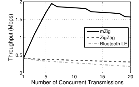
Figure 27: BLE simulation.
