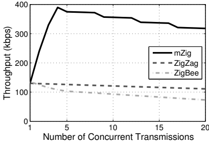
Figure 22: Throughput simulation.
