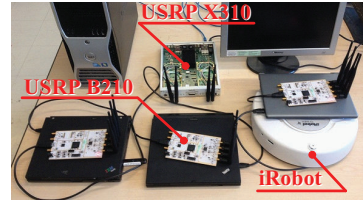
Figure 15: Testbed
