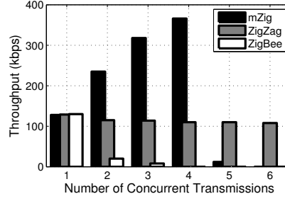
Figure 17: Comparison of schemes on throughput (without MAC).
