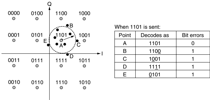
Figure 2-24. Gray-coded QAM-16.
