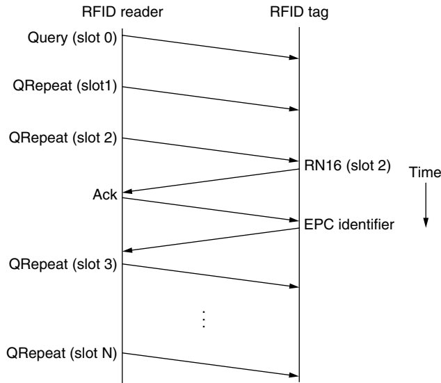
Figure 4-39. Example message exchange to identify a tag.
