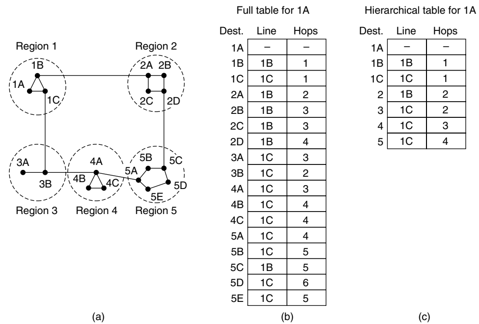
Figure 5-14. Hierarchical routing.
