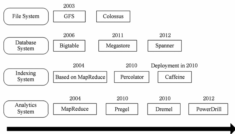
Fig. 4 Technology evolution in Google.
