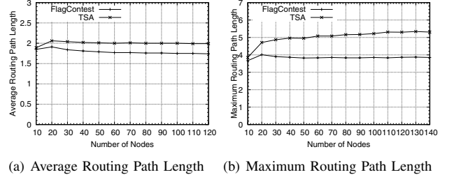
Fig. 8. Comparison of Average Routing Path Length and Maximum Routing Path Length in DG Networks between FlagContest and TSA.
