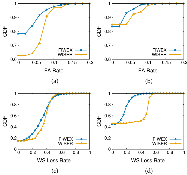
Fig. 8. CDF curves of FA Rate and WS Loss Rate. (a) 10 Sensors. (b) 30 Sensors. (c) 10 Sensors. (d) 30 Sensors.
