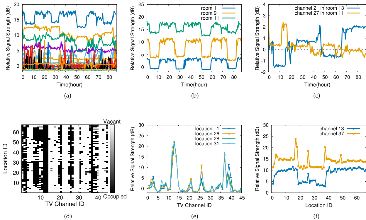
Fig. 1. Results of indoor white space measurement: long-time sensing and short-time sensing. (a) Relative signal strengths for 45 TV channels of room 11 in a 87.5-hour window. (b) TV channel 13 in room (1, 9, 11). (c) Two short term occupied channels. (d) Indoor white space availability map. (e) Location dependence. (f) Channel dependence.
