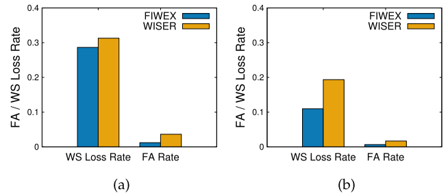
Fig. 7. Average FA rate, WS Loss Rate. (a) 10 Sensors. (b) 30 Sensors.
