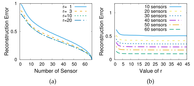
Fig. 11. Influence of r . (a) Different r . (b) Different number of sensors.
