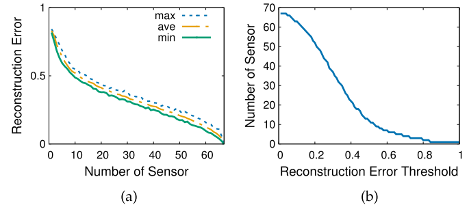
Fig. 14. Reconstruction error and the number of sensors. (a) Reconstruction error. (b) Number of sensors.
