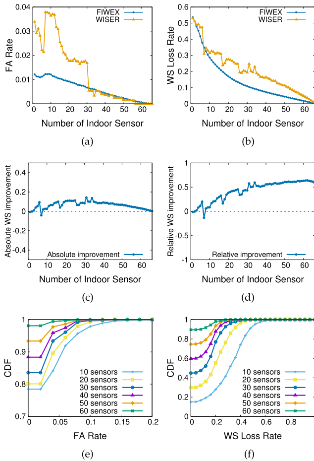
Fig. 9. Evaluation results on the number of sensors. (a) FA Rate. (b) WS Loss Rate. (c) Absolute WS improvement. (d) Relative WS improvement. (e) FA Rate CDF. (f) WS Loss Rate CDF.
