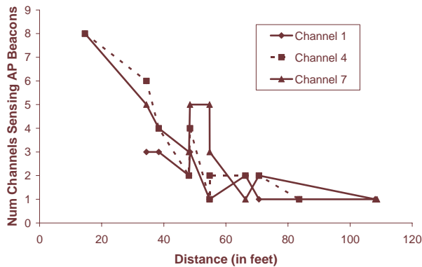
Figure 13: Overlapping channels heard relative to distance
