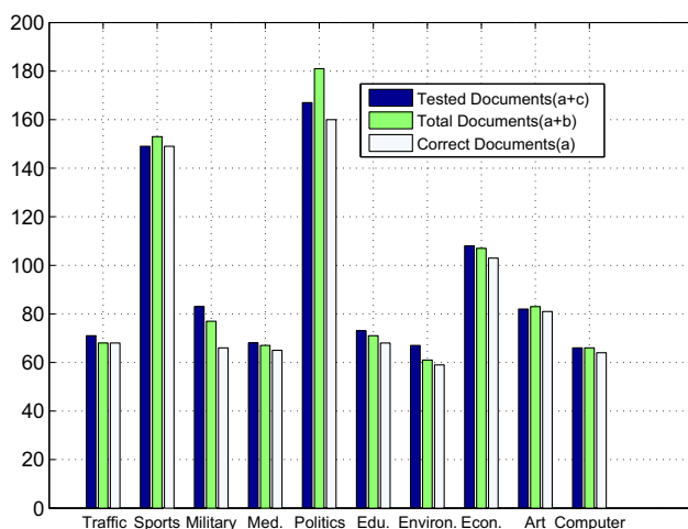
Fig. 12. The number of classified documents.
