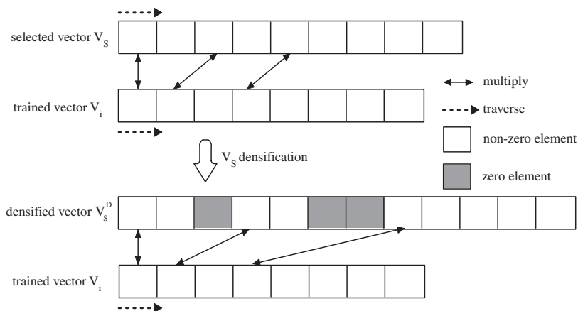
Fig. 1. Semi-sparse vector multiplication.
