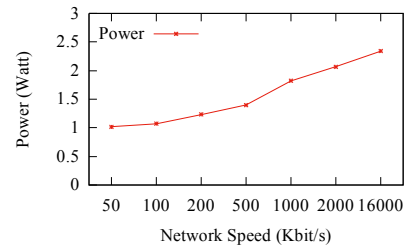
Fig. 4. Network Condition Effect
