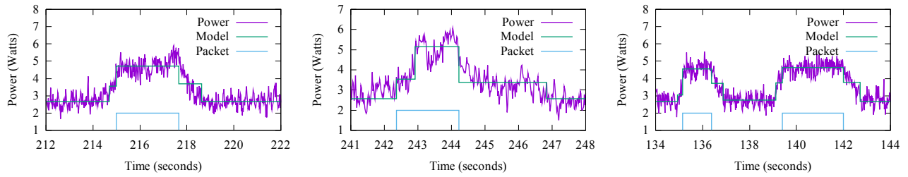
Fig. 3. Power Modeling
